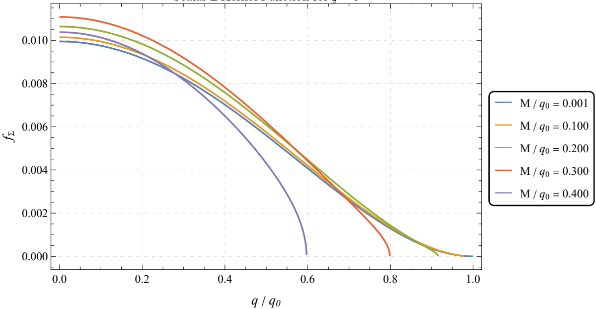
Scalar \Sigma Kernel Function for \xi = 0
